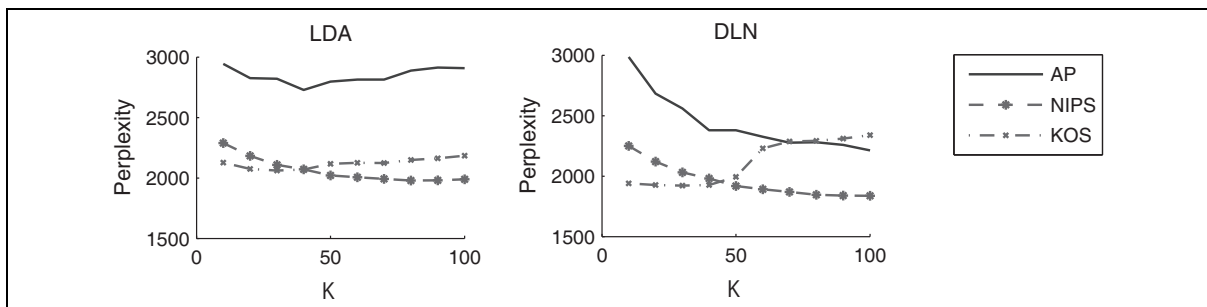
Fig. 5. Sensitivity of LDA and DLN against diversity, measured by perplexity as the number of topics increases. The testing sets were of same size and same document length in these experiments. Under the knowledge of Div_{NIPS} > Div_{AP} > Div_{KOS} , we can see that LDA performed inconsistently with respect to diversity; DLN performed much more consistently.
