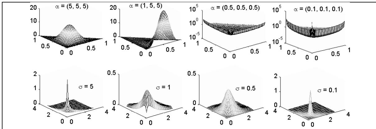
Fig. 2. Illustration of two distributions in the 2-dimensional space. The top row are the Dirichlet density functions with different parameter settings. The bottom row are the Lognormal density functions with parameters set as \mu = 0, \Sigma = \text{Diag}(\sigma) .
