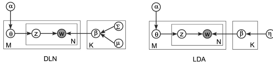
Fig. 3. Graphical model representations of DLN and LDA.
