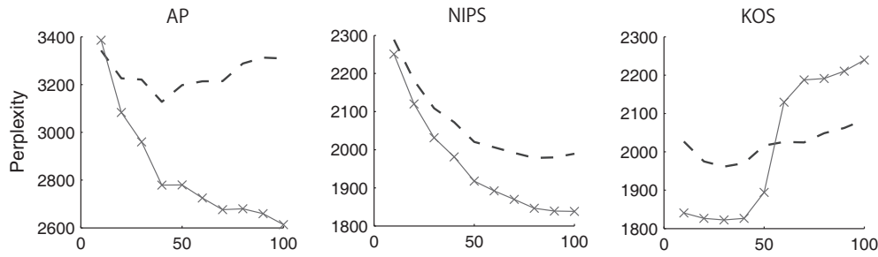
Fig. 4. Perplexity as the number of topics increases. Solid curves are DLN, dashed curves are LDA. The lower is the better.
