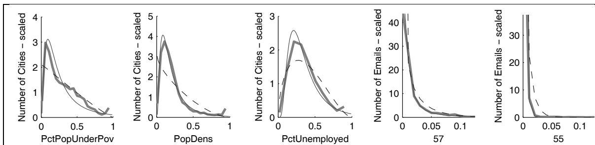
Fig. 1. Distributions of some attributes in Comm-Crime and SPAM. Bold curves are the histograms of the attributes. Thin curves are the best fitted Lognormal distributions; dashed curves are the best fitted Beta distributions.
