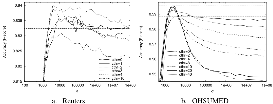
Figure 2. Best cth and \sigma combinations for Gaussian MAP estimation.
