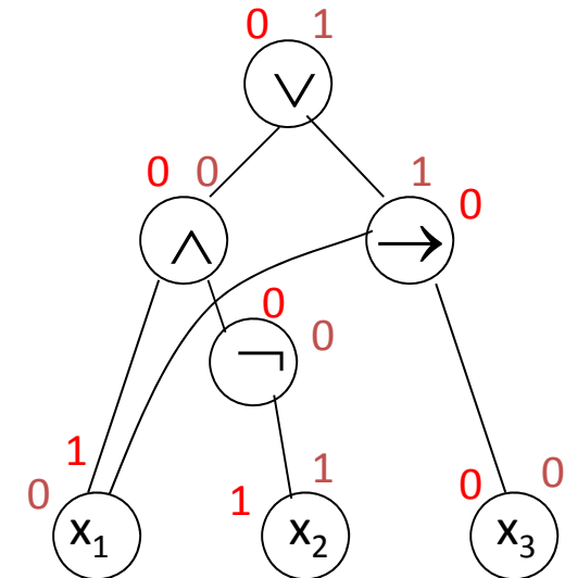
computation tree
