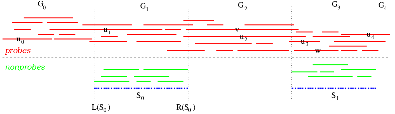
Figure 6: Segments and a decomposition of a probe interval graph
