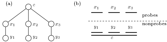
Figure 8: Enhanced probe interval and not strongly chordal graph
