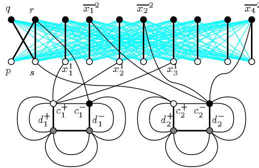
Figure 5: The reduction given C_1 = (x_1, x_2, x_3) and C_2 = (\bar{x}_1, \bar{x}_2, \bar{x}_4)
