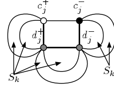
Figure 4: The gadget G(C_j)
