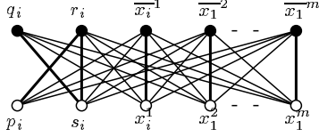
Figure 3: The gadget G(x_i)
