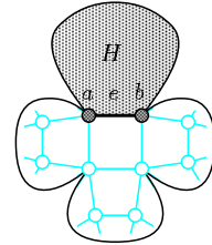
Figure 2: The graph obtained from H and S_\ell[a, b] by identifying the edge e = \{a, b\}
