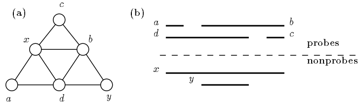
Figure 8: Enhanced probe interval and not strongly chordal graph
