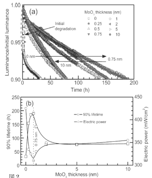
図2 FIG. 5. (a) Luminance/initial luminance-time characteristics of OLEDs with various thickness of MoO 3 HIL and (b) 90% lifetime and electric power vs MoO 3 thickness of OLEDs. All OLEDs were operated at constant dc current density of 50 mA/cm 2 .
