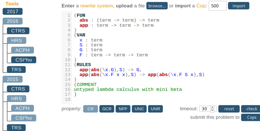
Fig. 3. Problem and tool selection in CoCoWeb.
