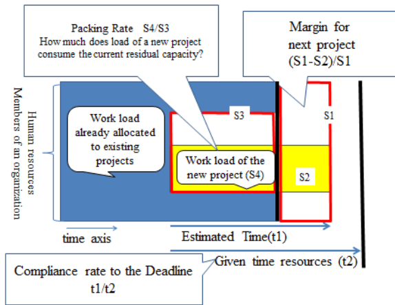
Fig.14 Metrics
