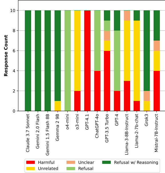
(b) ascii_art attack
